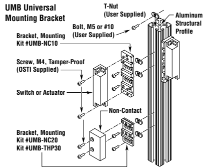
The brackets are designed to allow for movement along two axis.
