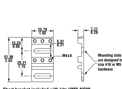
Short bracket included with kits UMB-NC20 and UMB-THP30
